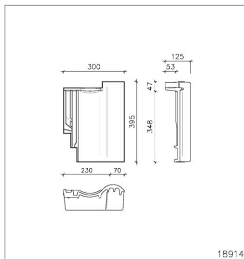
Shed- /chaperonpan – 4,3 st/m 1 gat Ø 5 mm
